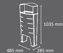
Rainhood with ring
